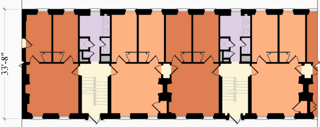
RENOVATED GROUND FLOOR – TIMOTHY DWIGHT
